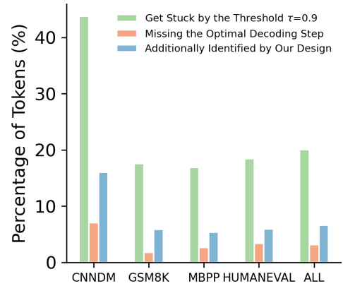
Figure 2: Quantifying Failure Modes of Static Thresholding.
