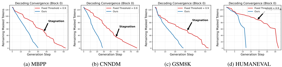
Figure 4: Comparison of decoding convergence between the static baseline (Fast-dLLM, red) and our method (blue) on four distinct tasks: CNN/DM, GSM8K, MBPP, HumanEval.
